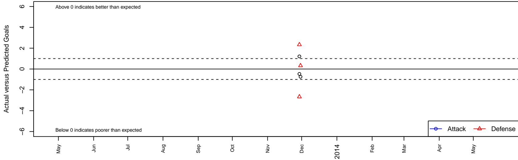
Freedom FC Blue G00 Dots are actual minus expected GF (blue circles) and GA (red triangles). Blue line is smoothed change in attack strength. Red is smoothed change in defense strength.
